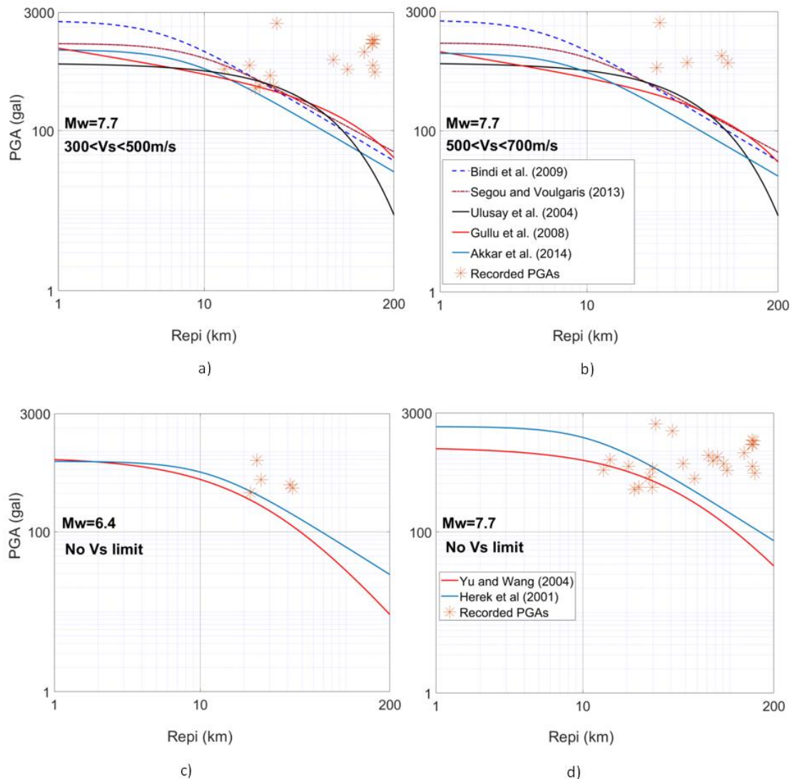
Figure 2. Comparison of the New Generation Attenuation (NGA) equations for a) M_w=7.7 and 300 < V_s < 500 \text{ m/s} , b) M_w=7.7 and 500 < V_s < 700 \text{ m/s} , c) M_w=6.4 and no V_s limit and d) M_w=7.7 and no V_s limit
