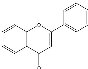
Figure 9. Flavone
