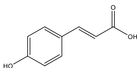
Figure 3. Coumaric Acid
